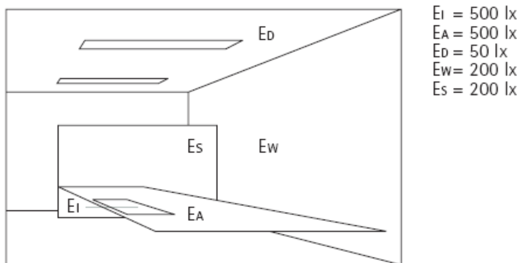
Fig. 1: Examples of brightness levels at different spots in a typical office room (worktable EA=500 lx)
